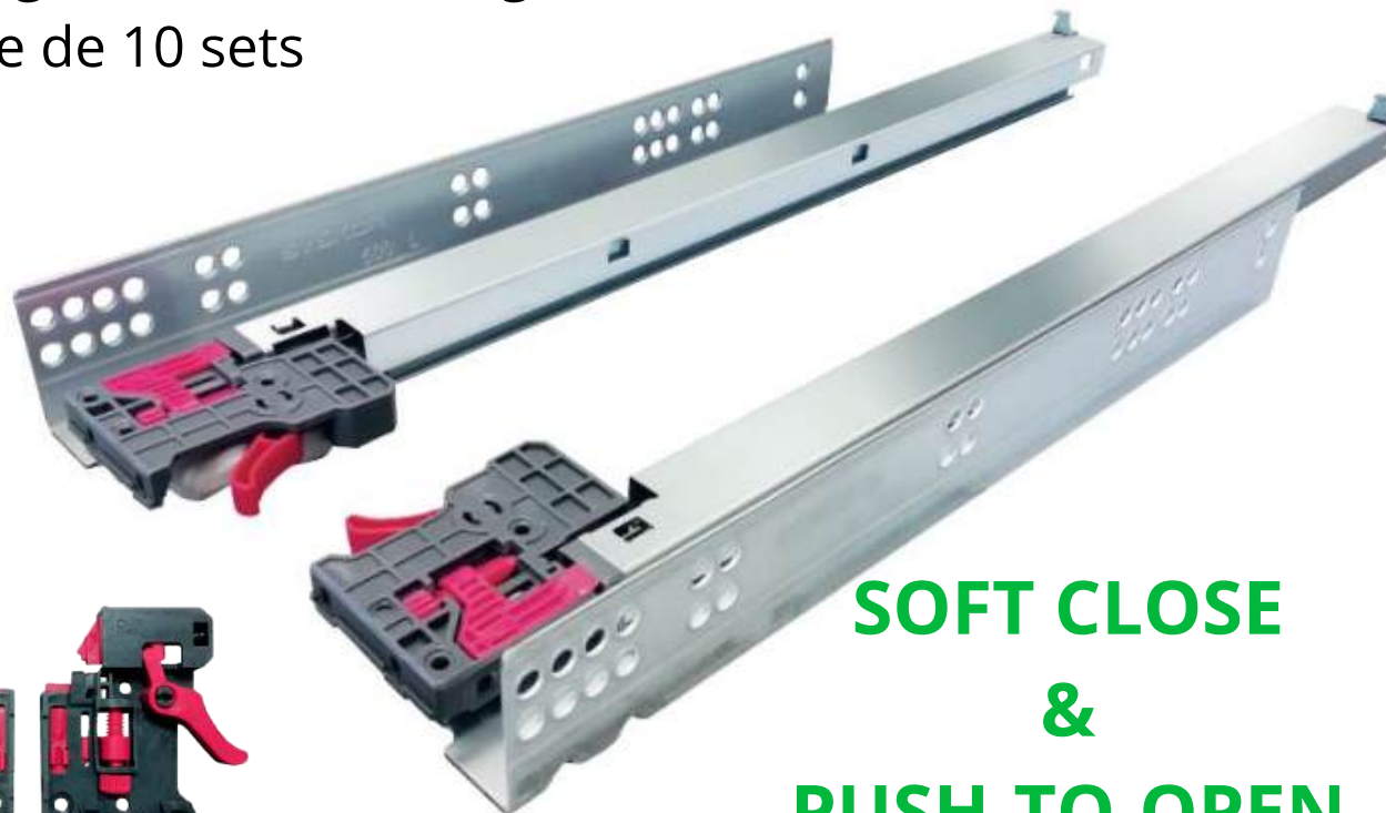
height regulation brackets for easy installation and adjustment
